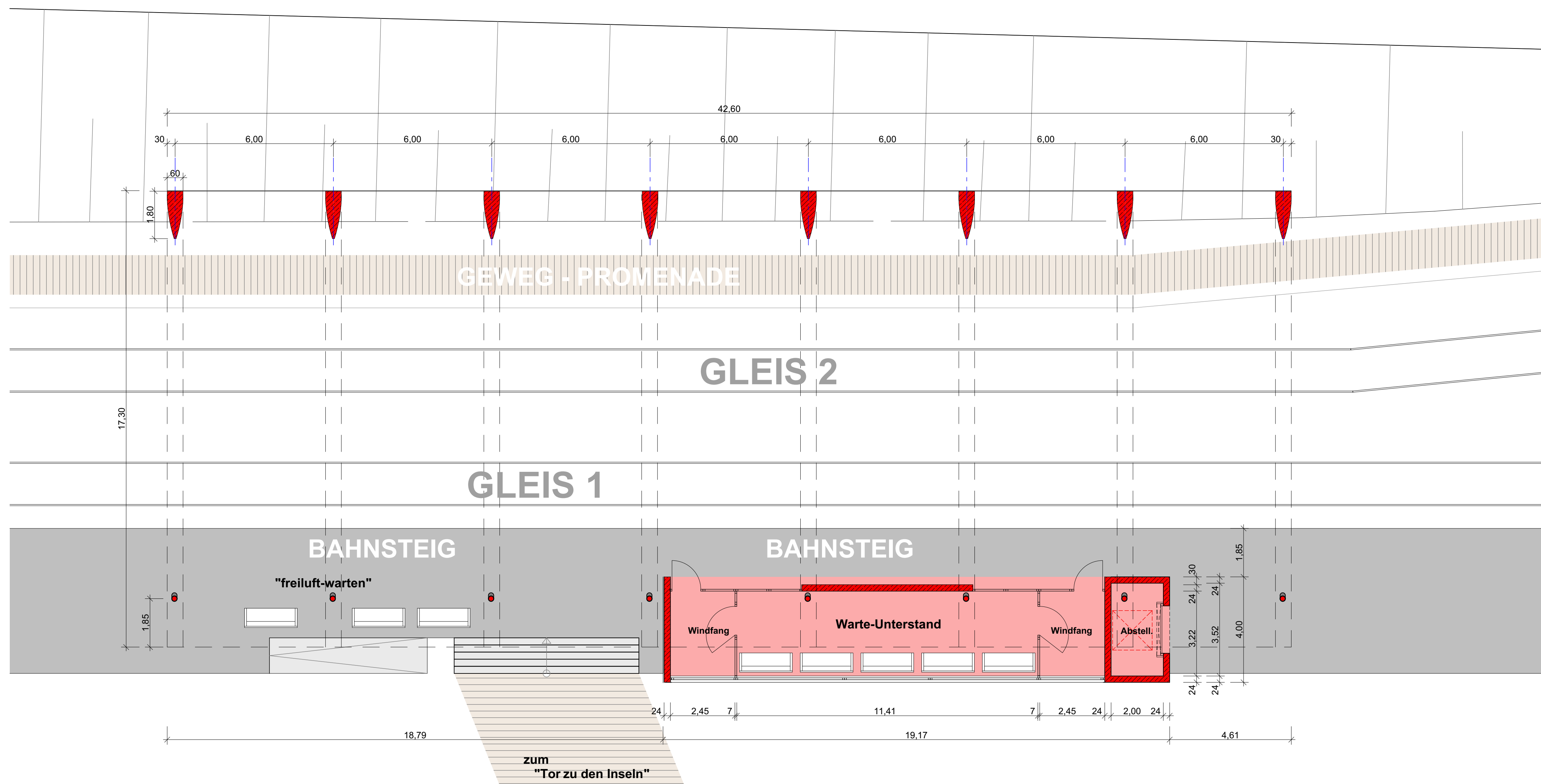
Grundriss_M. 1:100
